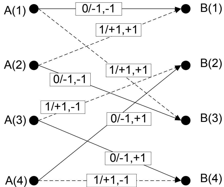
Figure. The trellis section
