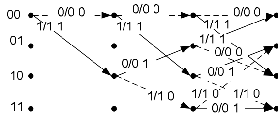
Figure 1. transition trellis of the encoder.
