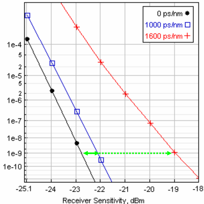
BER Receiver Sensitivity for different Dispersion Levels.
