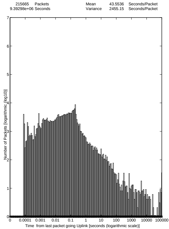
WWW traffic in WSs 5.8.-23.9.1996 27-Oct-96 The Distribution of Packet Interarrival Times (Up Packets) 3/3
