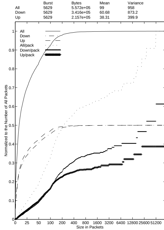
WWW traffic in WSs 5.8.-23.9.1996 27-Oct-96 The Cumulative Distribution of Bursts by their Size in Packets
