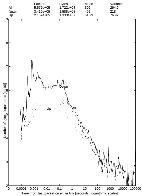
WWW traffic in WSs 5.8.-23.9.1996 27-Oct-96 The Distribution of IP-Bytes by Packet Interarrival Times
