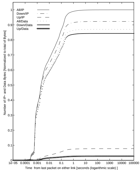
WWW traffic in WSs 5.8.-23.9.1996 27-Oct-96 The Cumulative Distribution of IP- and Data Byte by Packet
