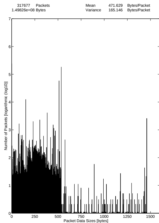
WWW traffic in WSs 5.8.-23.9.1996 27-Oct-96 The Distribution of Packets by Data Sizes (All Packets)
