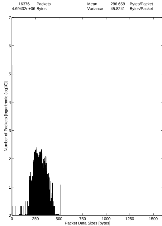
WWW traffic in WSs 5.8.-23.9.1996 27-Oct-96 The Distribution of Packets by Data Sizes (Up Packets)
