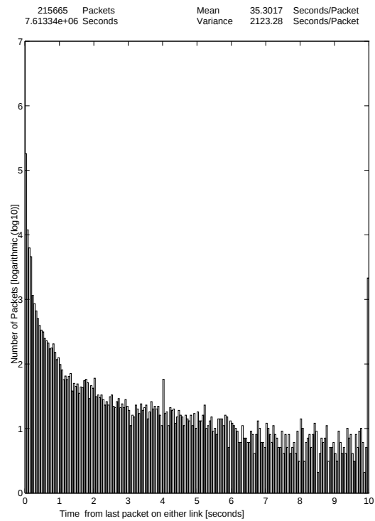
WWW traffic in WSs 5.8.-23.9.1996 27-Oct-96 The Distribution of Packet Interarrival Times (Up Packets) 1/3
