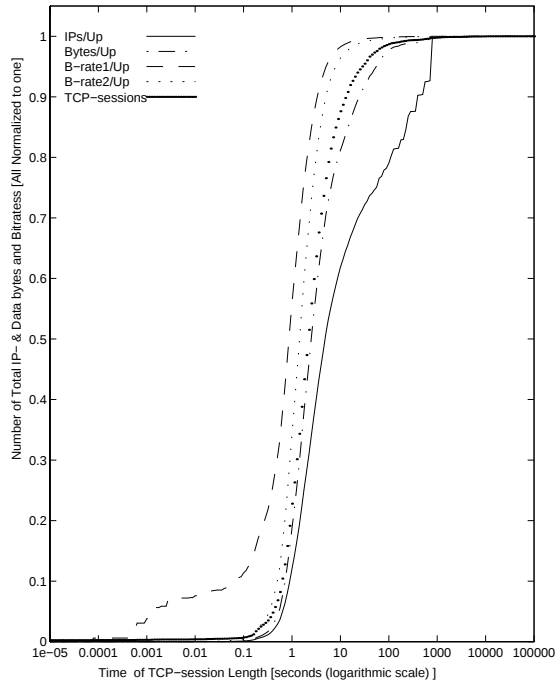
WWW traffic in WSs 5.8.-23.9.1996 27-Oct-96 The Cumulative Distribution of Total IP- & Data bytes and Bitrates by TCP-session Length
