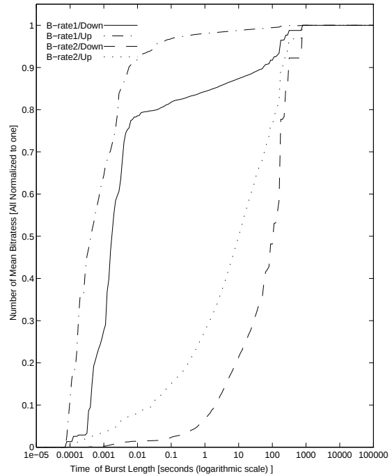
WWW traffic in WSs 5.8.-23.9.1996 27-Oct-96 The Cumulative Distribution of Mean Bitrates by Burst Length
