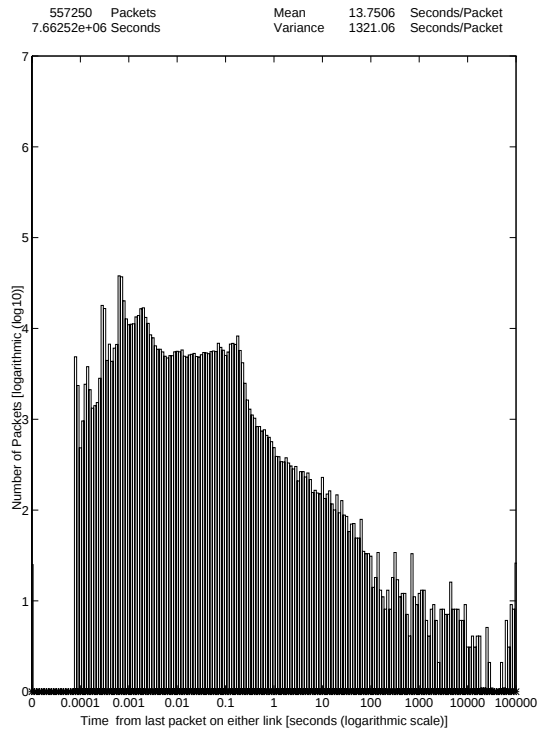
WWW traffic in WSs 5.8.-23.9.1996 27-Oct-96 The Distribution of Packet Interarrival Times (All Packets) 3/3
