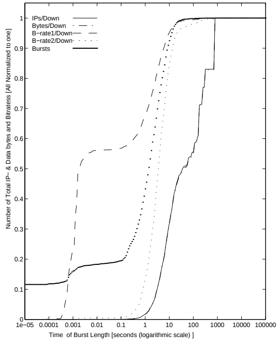
WWW traffic in WSs 5.8.-23.9.1996 27-Oct-96 The Cumulative Distribution of Total IP- & Data bytes and Bitrates by Burst Length
