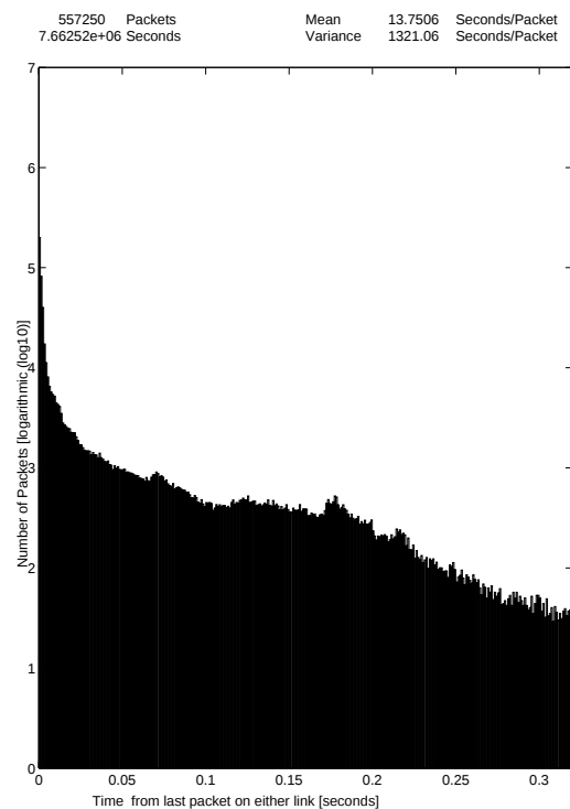
WWW traffic in WSs 5.8.-23.9.1996 27-Oct-96 The Distribution of Packet Interarrival Times (All Packets) 2/3
