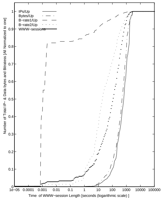
WWW traffic in WSs 5.8.-23.9.1996 27-Oct-96 The Cumulative Distribution of Total IP- & Data bytes and Bitrates by WWW-session Length
