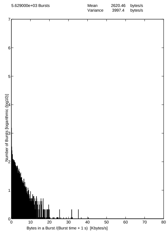
WWW traffic in WSs 5.8.-23.9.1996 27-Oct-96 The Distribution of Bursts by Average Bitrate (Down Packets) A Burst (= arrival time < 2 s)
