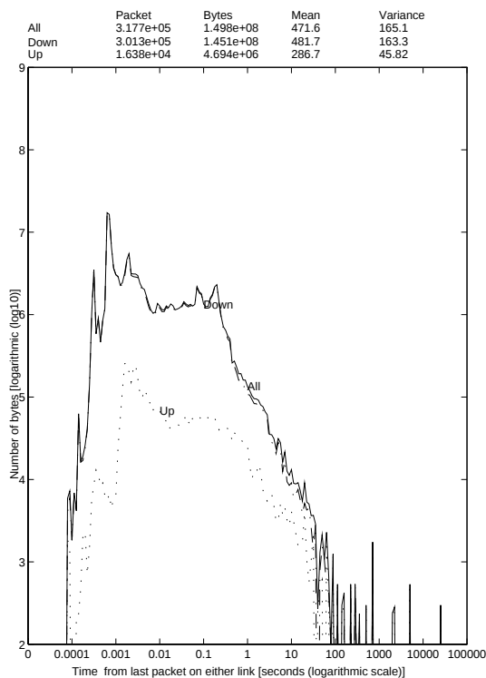
WWW traffic in WSs 5.8.-23.9.1996 27-Oct-96 The Distribution of Data Bytes by Packet Interarrival Times
