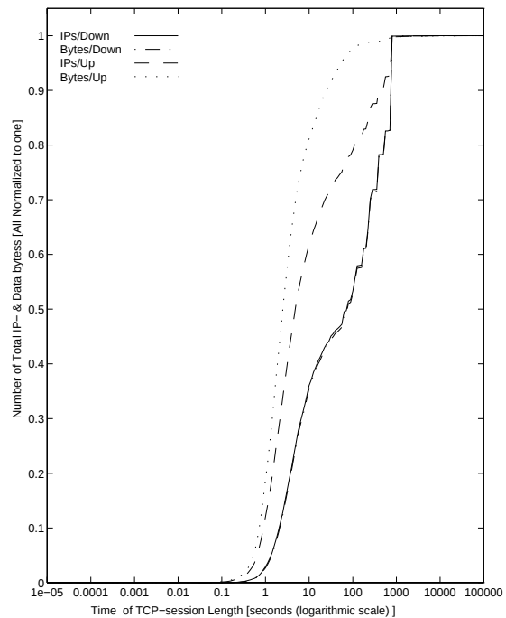
WWW traffic in WSs 5.8.-23.9.1996 27-Oct-96 The Cumulative Distribution of Total IP- & Data bytes by TCP-session Length
