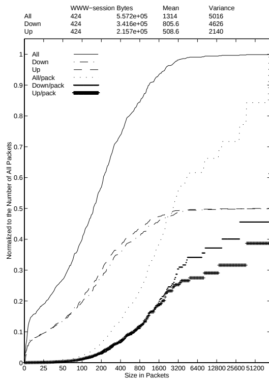
WWW traffic in WSs 5.8.-23.9.1996 27-Oct-96 The Cumulative Distribution of WWW-sessions by their Size in Packets
