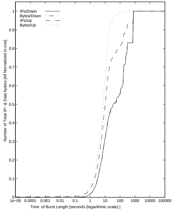
WWW traffic in WSs 5.8.-23.9.1996 27-Oct-96 The Cumulative Distribution of Total IP- & Data bytes by Burst Length
