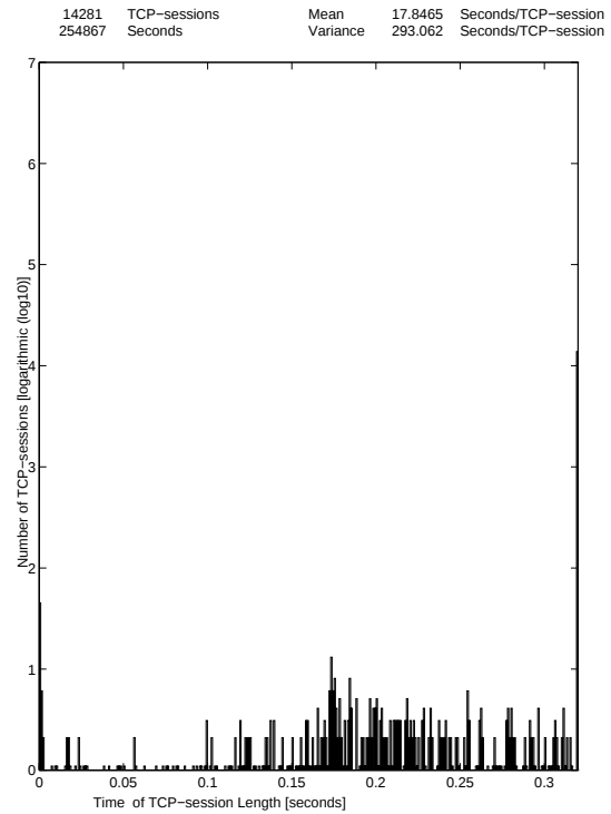
WWW traffic in WSs 5.8.-23.9.1996 27-Oct-96 The Distribution of TCP-session Length 2/3
