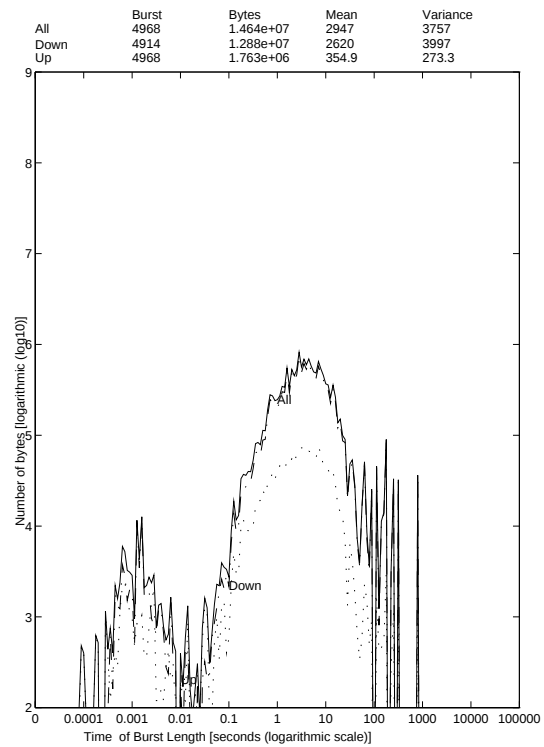
WWW traffic in WSs 5.8.-23.9.1996 27-Oct-96 The Distribution of Bitrate2 in Bytes by Burst Length
