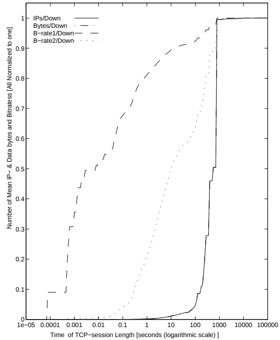
WWW traffic in WSs 5.8.-23.9.1996 27-Oct-96 The Cumulative Distribution of Mean IP- & Data bytes and Bitrates by TCP-session Length
