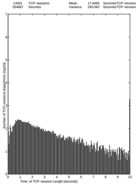
WWW traffic in WSs 5.8.-23.9.1996 27-Oct-96 The Distribution of TCP-session Length 1/3
