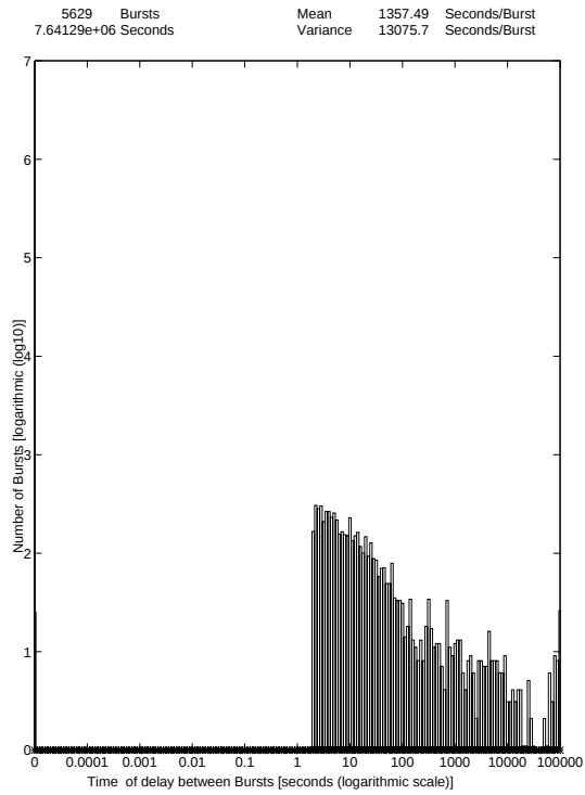
WWW traffic in WSs 5.8.-23.9.1996 27-Oct-96 The Distribution of delay between Bursts 3/3
