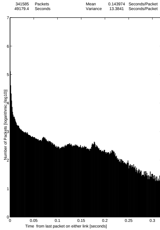
WWW traffic in WSs 5.8.-23.9.1996 27-Oct-96 The Distribution of Packet Interarrival Times (Down Packets) 2/3
