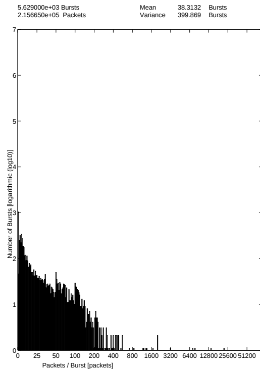
WWW traffic in WSs 5.8.-23.9.1996 27-Oct-96 The Distribution of Bursts by Size (Up Packets) A Burst (= arrival time < 2 s)
