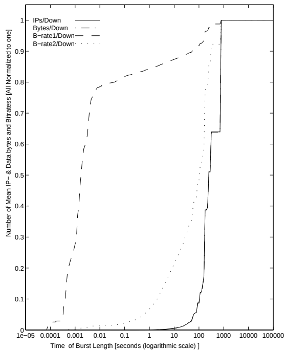
WWW traffic in WSs 5.8.-23.9.1996 27-Oct-96 The Cumulative Distribution of Mean IP- & Data bytes and Bitrates by Burst Length
