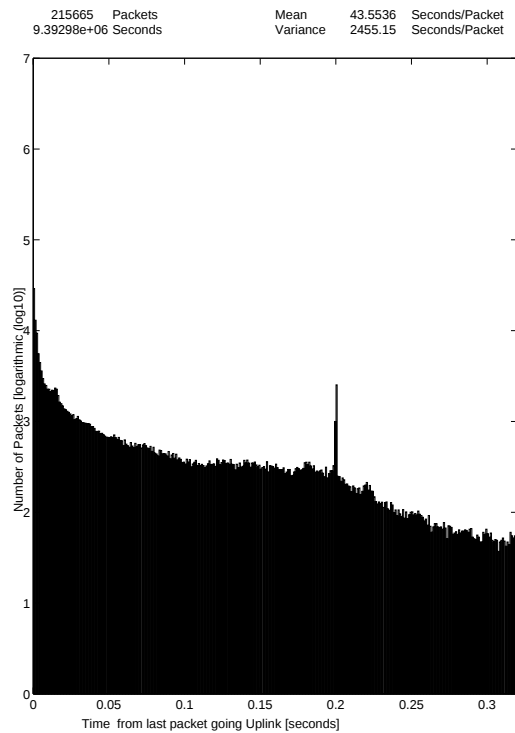
WWW traffic in WSs 5.8.-23.9.1996 27-Oct-96 The Distribution of Packet Interarrival Times (Up Packets) 2/3
