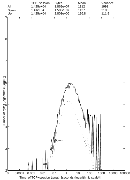
WWW traffic in WSs 5.8.-23.9.1996 27-Oct-96 The Distribution of Bitrate2 in Bytes by TCP-session Length
