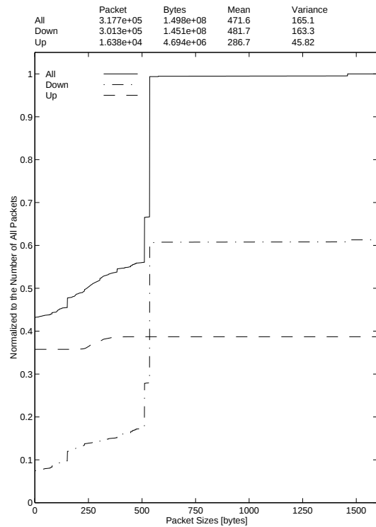
WWW traffic in WSs 5.8.-23.9.1996 27-Oct-96 The Cumulative Distribution of Packet by their Data Sizes
