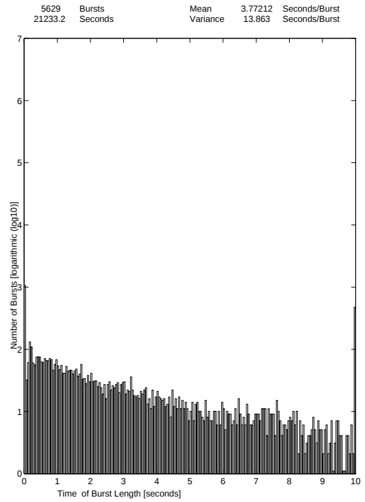
WWW traffic in WSs 5.8.-23.9.1996 27-Oct-96 The Distribution of Burst Length 1/3
