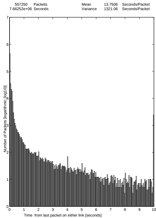
WWW traffic in WSs 5.8.-23.9.1996 27-Oct-96 The Distribution of Packet Interarrival Times (All Packets) 1/3
