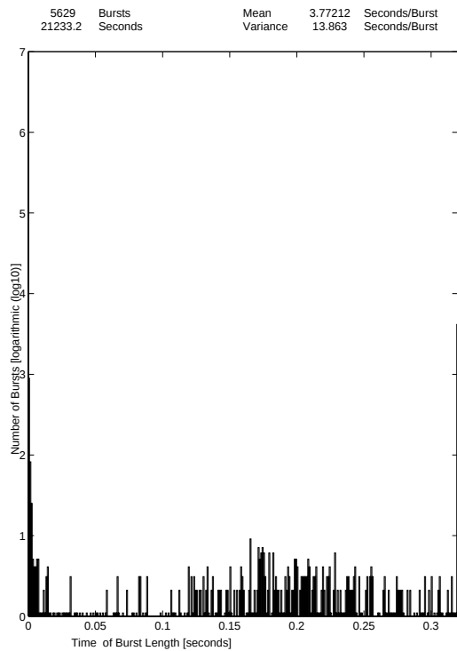
WWW traffic in WSs 5.8.-23.9.1996 27-Oct-96 The Distribution of Burst Length 2/3
